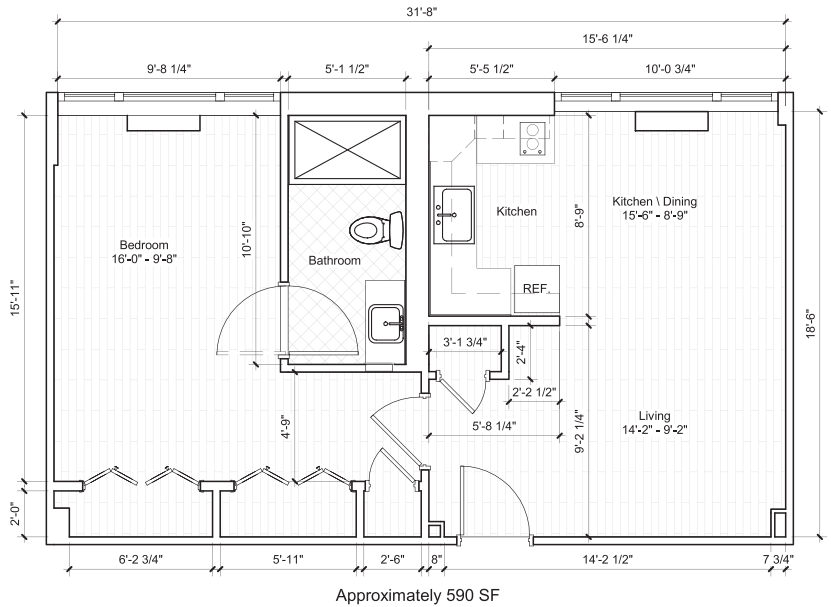
Standard 1 Bedroom Floorplan
